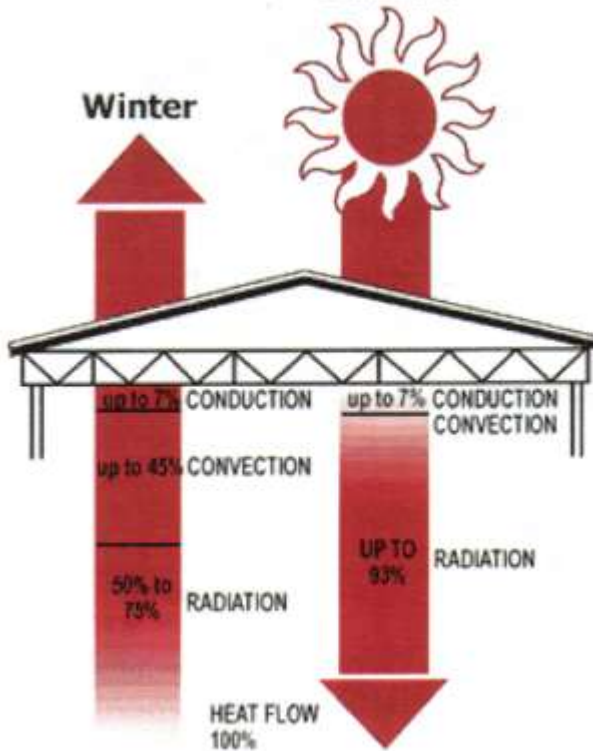
Radiant Foil Barrier Conductivity
